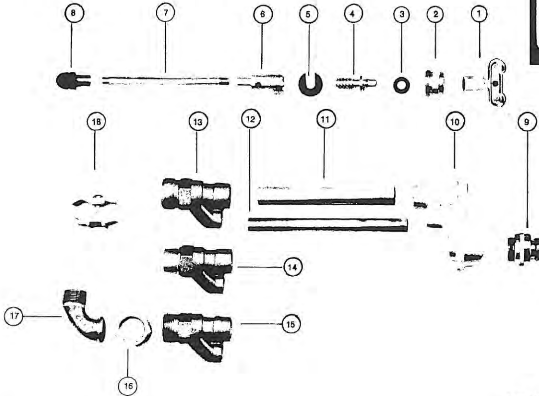
PART NO. 504XX— Operating Rod
