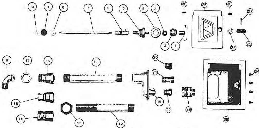
Woodford Freeless Model 90
