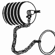
RUBBER INFLATABLE TEST PLUG C4851 - 1-1/4" - 1-1/2" C4852 - 2" C4853 - 3" C4854 - 4"
