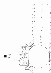
CHERNE CLEAN-SEAL Inflatable Test Plug C5522 - 2" C5523 - 3" C5524 - 4"
