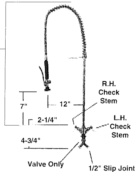
C3255 2990 Standard Spray Valve.
