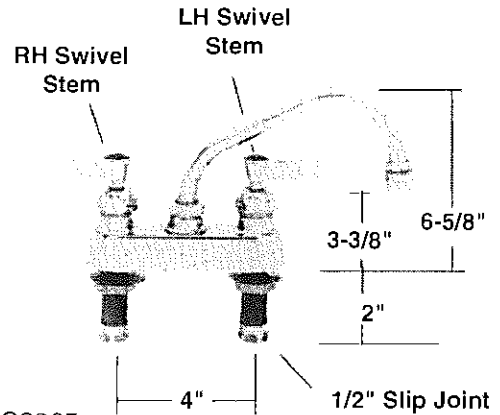
3511 C3265 Faucet with 8" Spout. Consists of: 3500 C3264 4" Deck Faucet L/S 3961 C3266 8" Swing Spout
