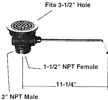
10758 C3226 Rotary Waste Valve with flat strainer.
