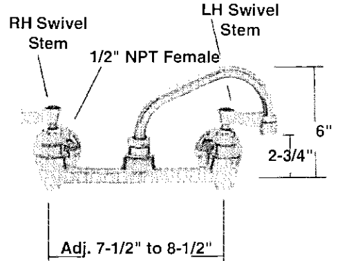
Faucet with 8" Spout. Consists of: 3200 C3262 Wall Mount Valve 3961 C3266 8" Swing Spout
